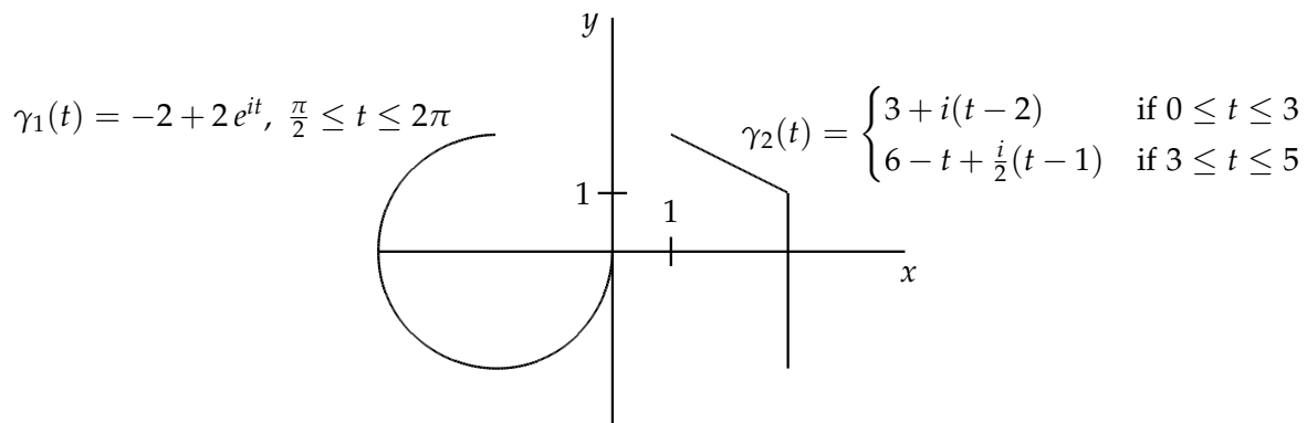
Figure 1.8: Two paths and their parametrizations; \gamma_1 is smooth and \gamma_2 is continuous and piecewise smooth.
